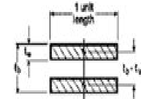
Double Sided Partial Penetration Groove Weld
