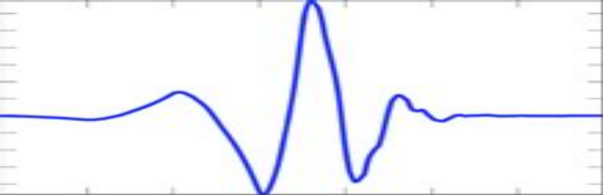
(a) db Wavelet
