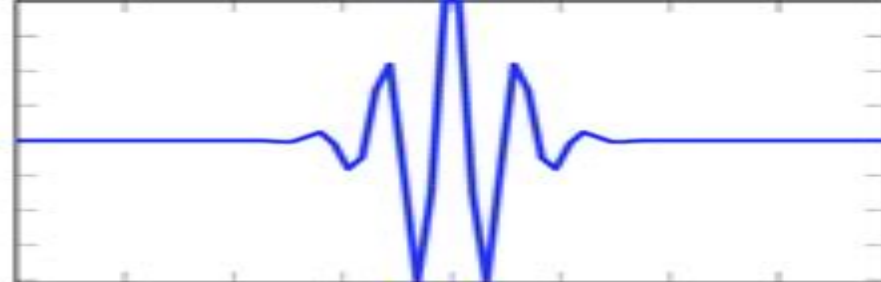
(b) Morlet Wavelet
