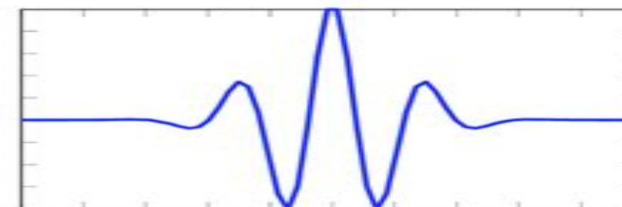
(g) Gaussian Wavelet
