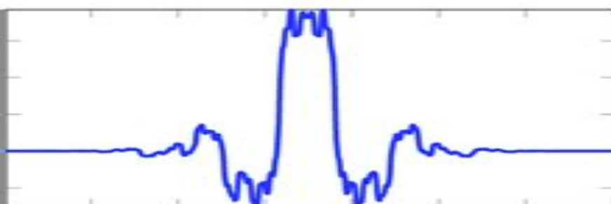
(c) Biorthogonal Wavelet
