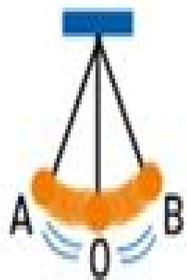
Oscillatory Motion
