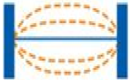
Vibratory Motion
