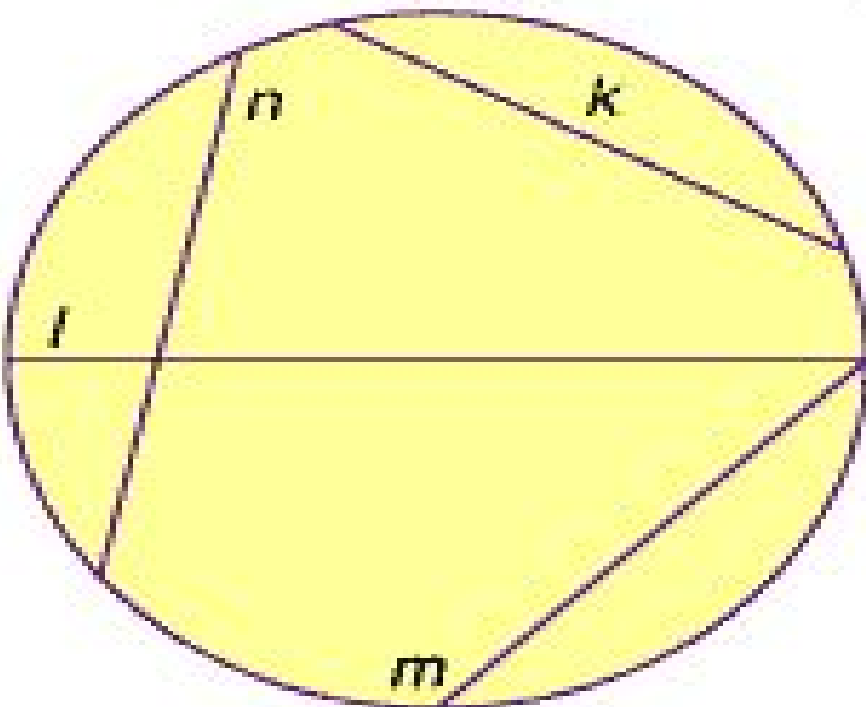
Klein-Beltrami model
