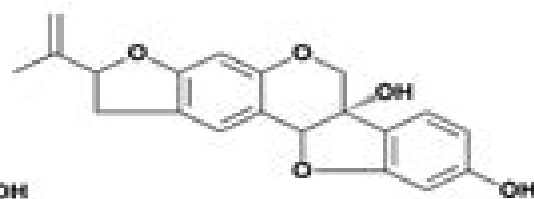
Phaseollidin (12)
