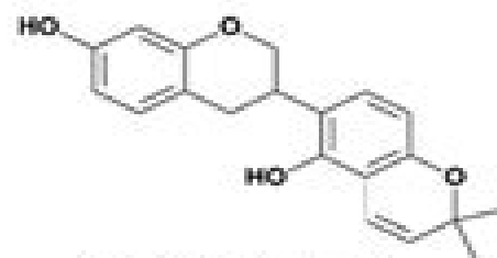
Phaseollinisoflavan (9)
