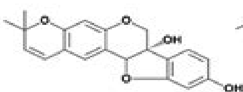
(+)-Glyceollin II (15)
