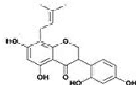
Kievitone (13)
