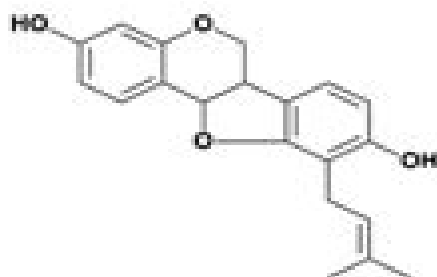
Phaseollidin (12)
