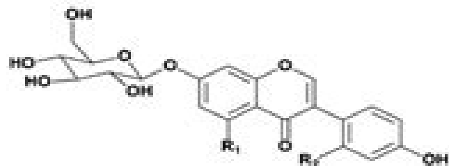
R 1 = R 2 = H; Daidzin (3)
