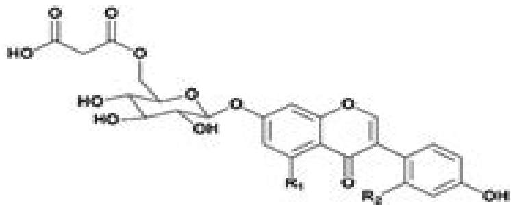
R 1 = R 2 = H; 6''-O-Malonyl-daidzin (1)
