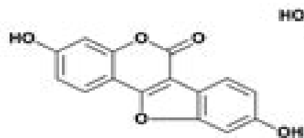
Coumestrol (10)
