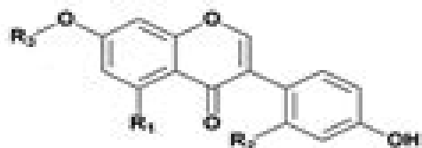
R 1 = R 2 = R 3 = H; Daidzein (5)
