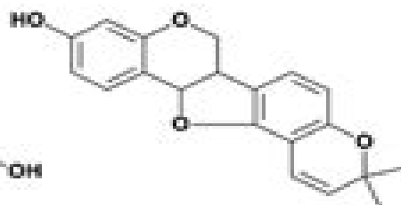
Phaseollin (11)
