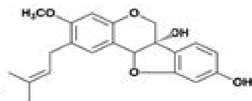
(+)-Glyceollin IV (17)
