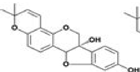
(+)-Glyceollin I (14)
