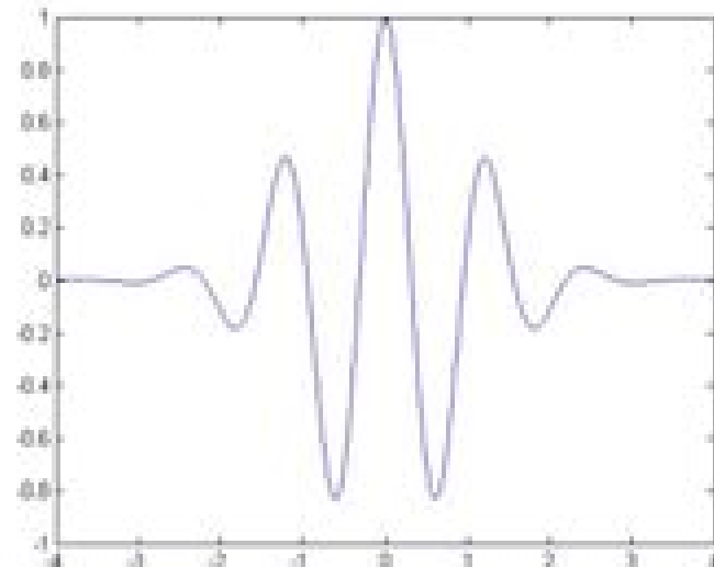
Morlet wavelet
