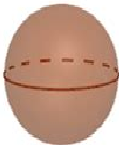
Sphere
