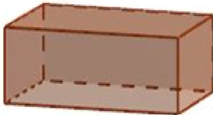
Rectangular prism
