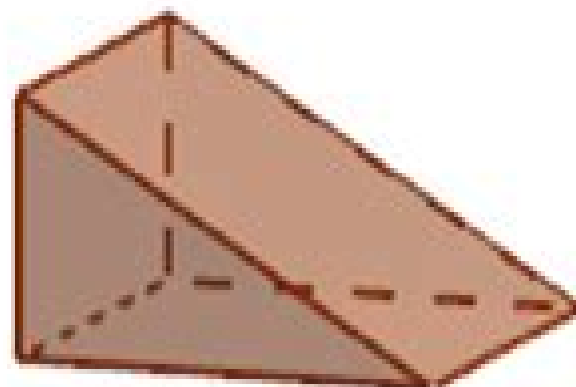
Triangular prism
