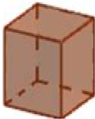
Cube
