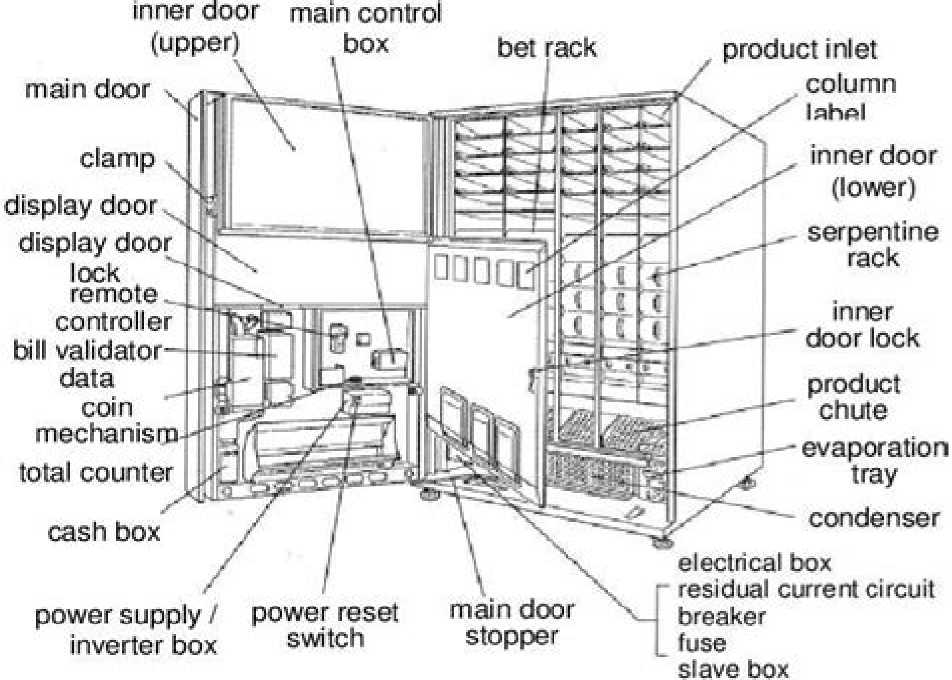
Fig 3.5 Interior of a Can or Bottle Vending
