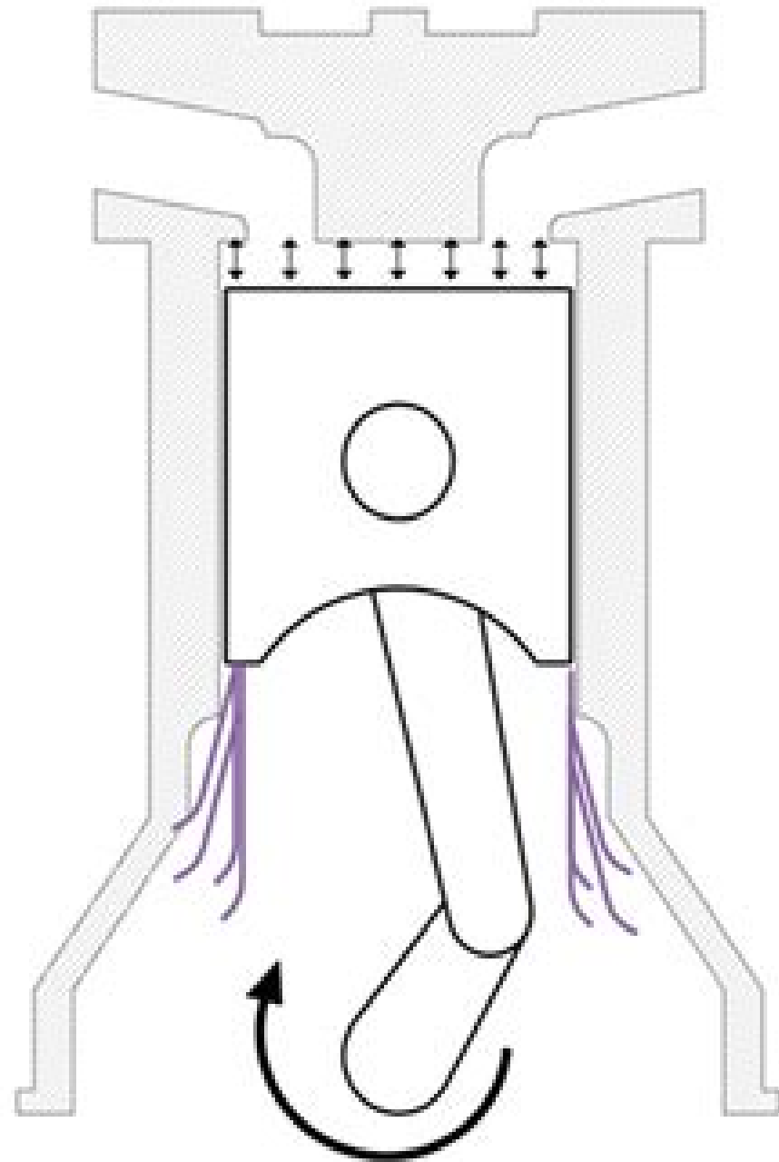
Compression Stroke Blow-By
