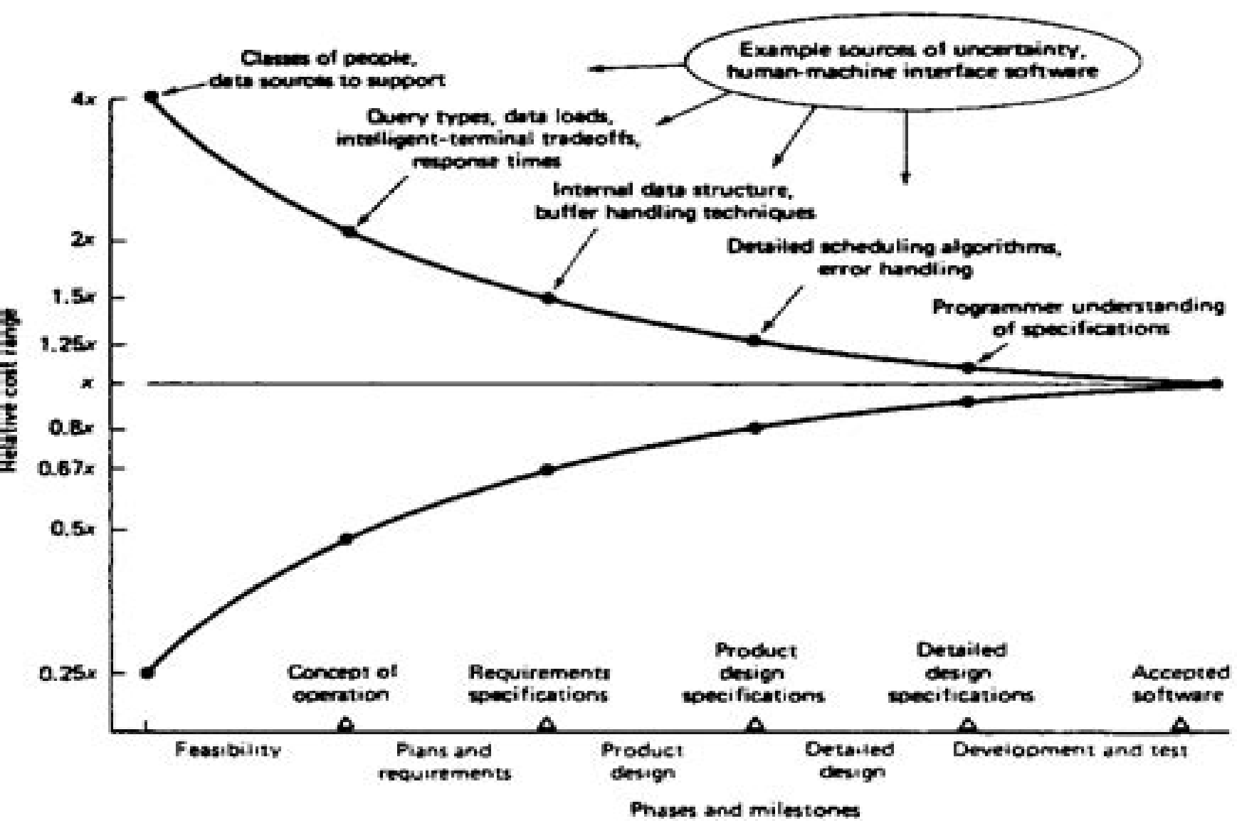
Fig. 3. Software cost estimation accuracy versus phase.
