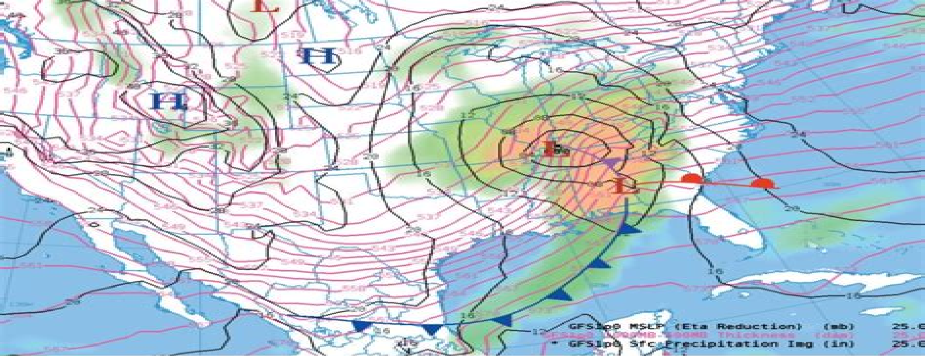
Above: GFS sea-level pressure and 1000-500 hPa thickness valid for 25 Jan 2023 at 1200 UTC. The thickness contours (red lines) represent a sort of averaged temperature in the lower and middle tropopause. The size of the boxes formed by the juxtaposition of thickness and sea-level pressure lines is, approximately, inversely proportional to the magnitude of thermal advection. (AWIPS-II)
