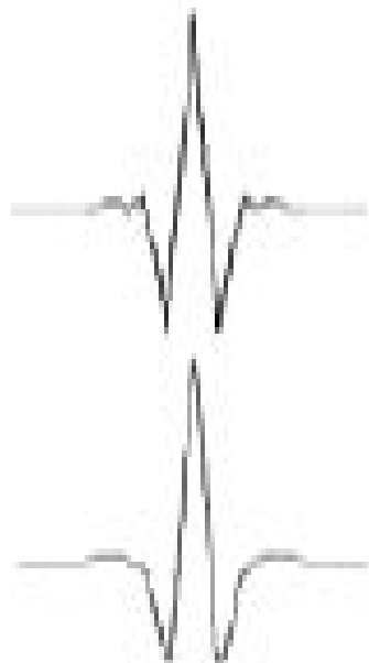
Biorthogonal
