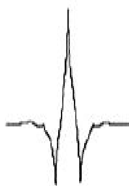
Coiflet
