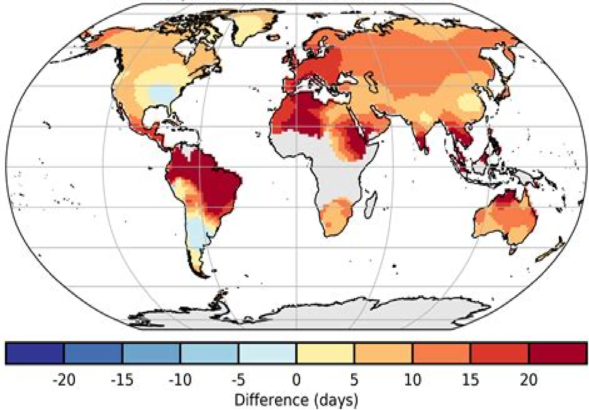
Warm Days, Difference (1981-2010) - (1951-1980)
