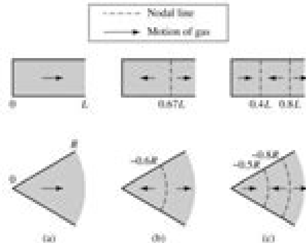
Standing sound waves in an organ pipe.
