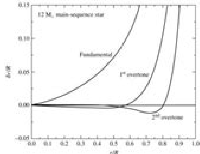
Radial modes for a pulsating star
