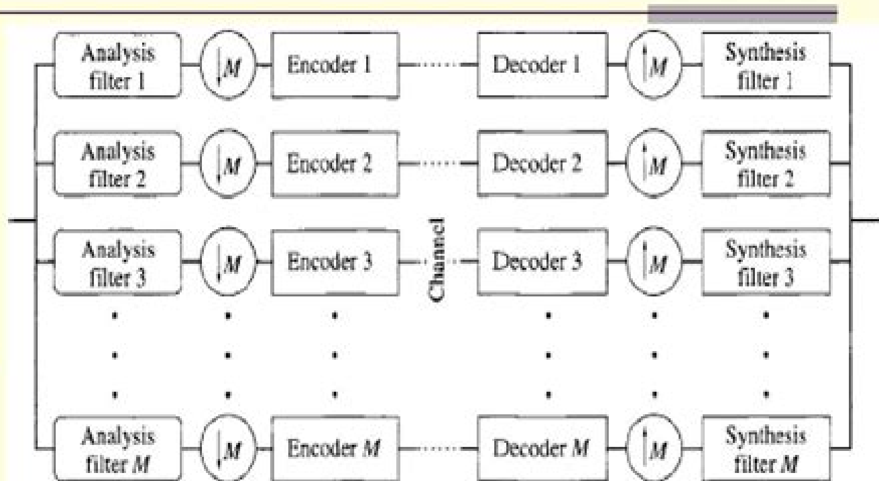
FIGURE 14.7 Block diagram of the subband coding system.
