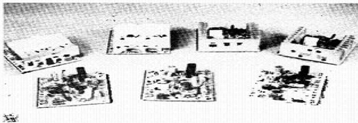
Fig. 1—Modules used in vertical circuitry in the Zenith J line of color TV. Top four modules are DC-coupled, and bottom three are AC-coupled modules.
